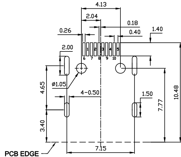
SUGGESTED PCB LAYOUT TOP VIEW SCALE: 2:1
